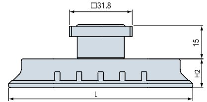
32 Square mounting
