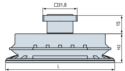
32 Square mounting
